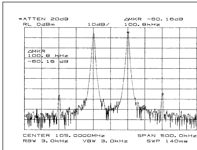
Figure 4. Mixer With High Side LO (IIP3 = +20 dBm, Input Power = -10 dBm)
