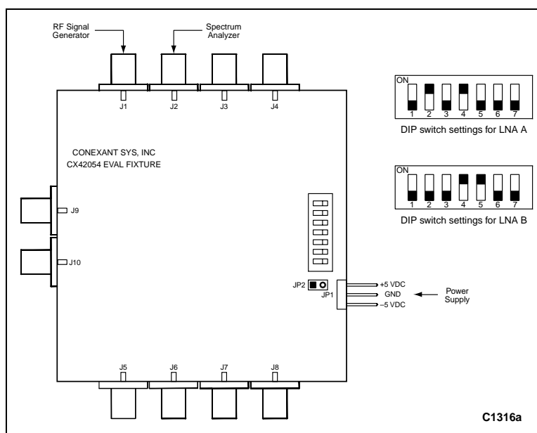
Figure 12. CX42054 Evaluation Board LNA Testing Configuration
