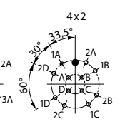
Drilling diagram for 60° indexing angle
