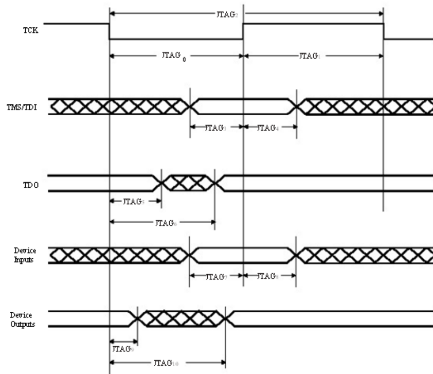
Figure 8-5: JTAG Timings
