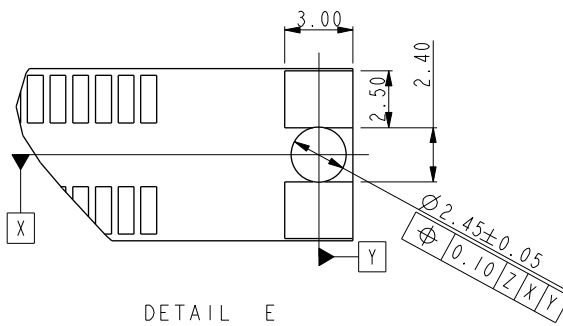
Center smt holdown type
