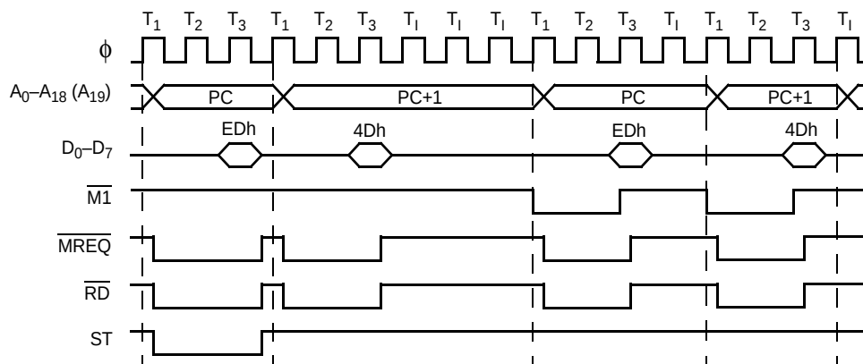
Figure 77. RETI Instruction Sequence with \text{M1E}=0
