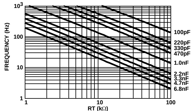
FIGURE 4. RESISTANCE FOR CT CAPACITOR VALUES GIVEN
