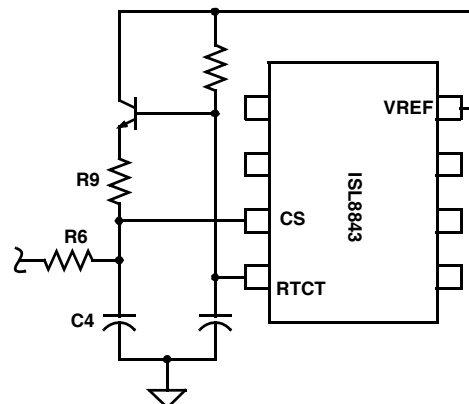
FIGURE 6. SLOPE COMPENSATION
