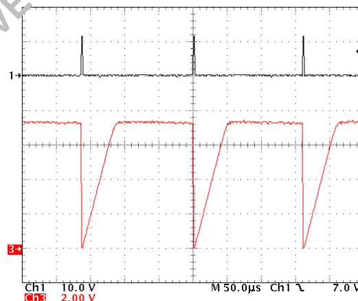
Figure 23. CT Voltage at No Load Condition
