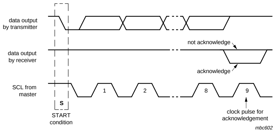
Fig 16. Acknowledgement on the I 2 C-bus
