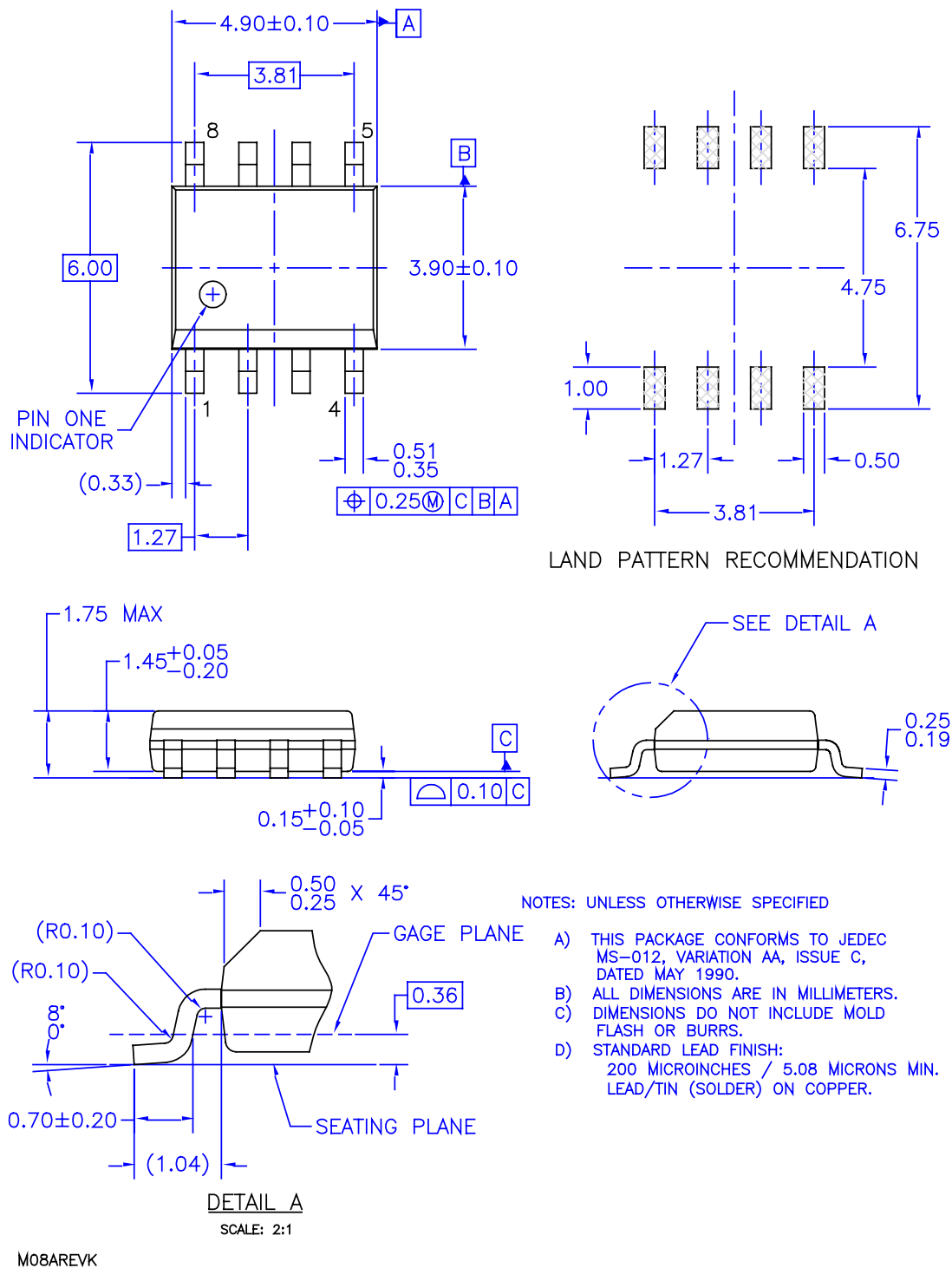
Figure 29. 8-Lead Small Outline Package (SOP)
