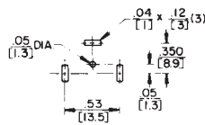
Recommended PC Board Layout (Component Side)
