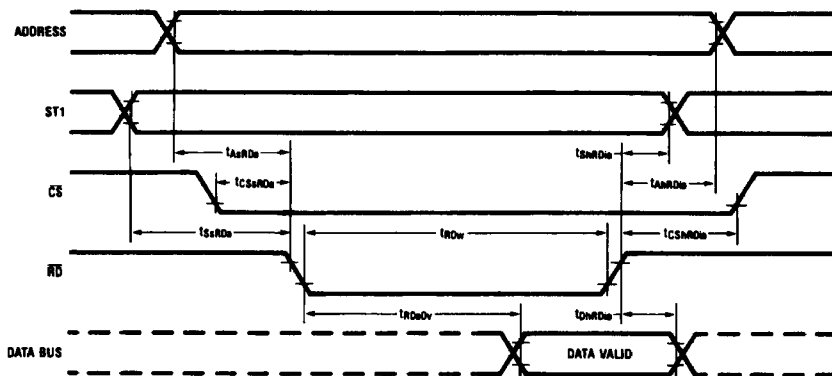
FIGURE 4-3. READ/INTA Cycle
