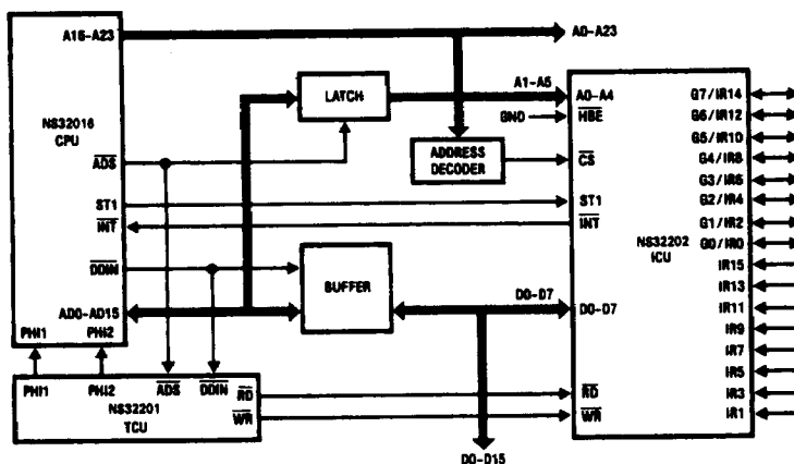
FIGURE 2-2. Interrupt Control Unit Connections in 8-Bit Bus Mode
