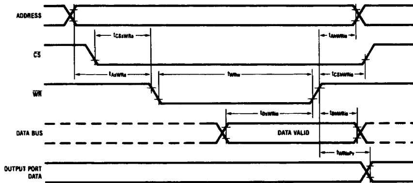
FIGURE 4-4. Write Cycle
