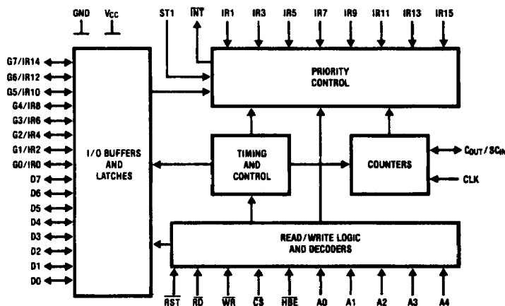
FIGURE 1-1. NS32202 ICU Block Diagram
