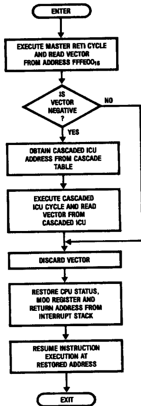
FIGURE 2-6. CPU Return from Interrupt Sequence
