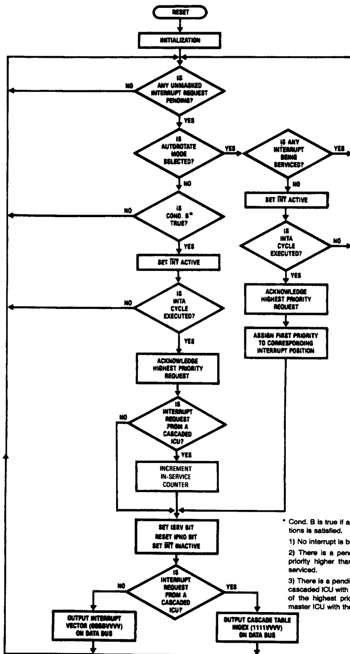
FIGURE 2-7. ICU Interrupt Acknowledge Sequence
