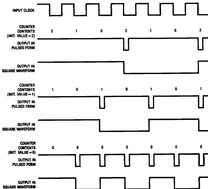
FIGURE 1-2. Counter Output Signals in Pulsed Form and Square Waveform for Three Different Initial Values
