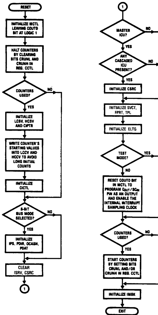
FIGURE 3-3. Recommended ICU's Initialization Sequence
