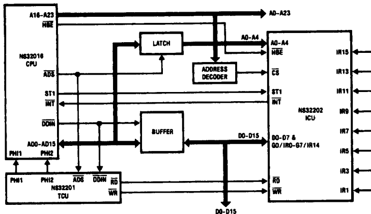
FIGURE 2-1. Interrupt Control Unit Connections in 16-Bit Bus Mode
