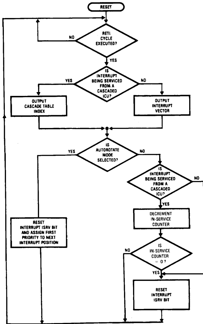
FIGURE 2-8. ICU Return from Interrupt Sequence
