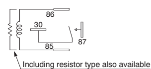
Schematic (Bottom view)
