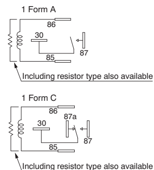
Schematic (Bottom view)
