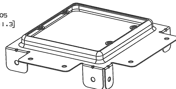
ISOMETRIC VIEW
