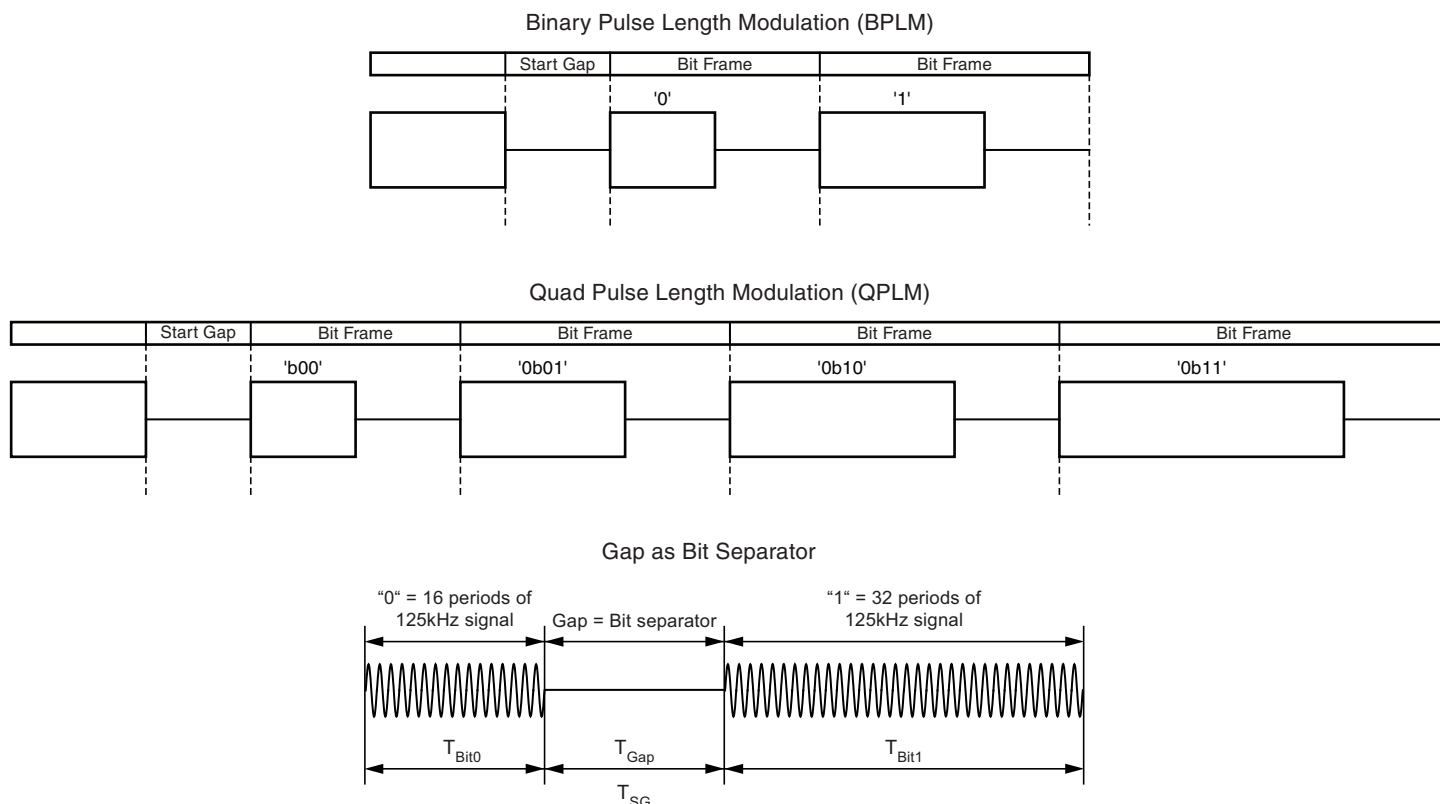
Figure 2-6. Downlink
