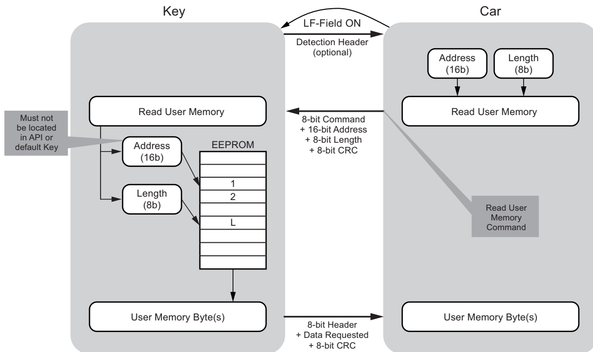
Figure 3-3. Read Memory
