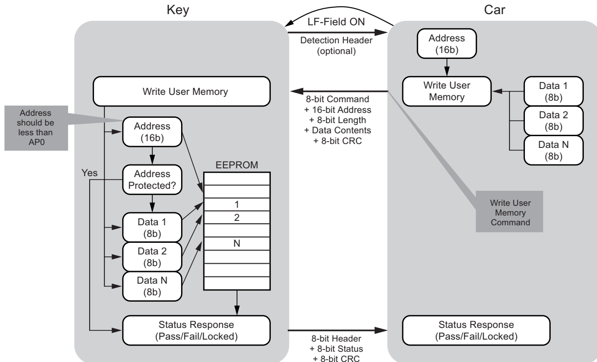
Figure 3-4. Write Memory
