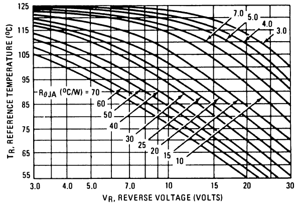
FIGURE 2 – MAXIMUM REFERENCE TEMPERATURE – 1N5824
