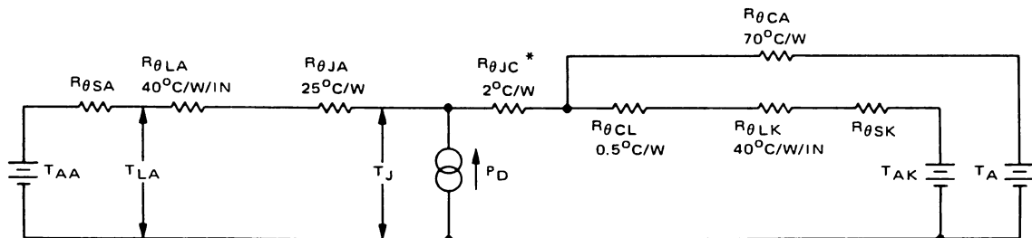
FIGURE 6 – APPROXIMATE THERMAL CIRCUIT MODEL
