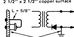
Board Ground Plane
