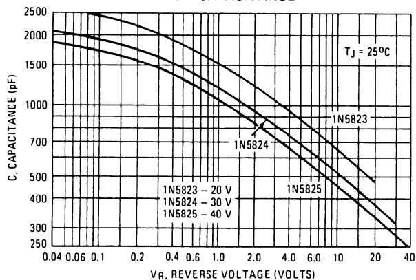
FIGURE 10 – CAPACITANCE
