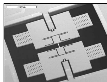
Figure 1.2 SAR10 Element structure
