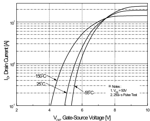
Figure 2. Transfer Characteristic
