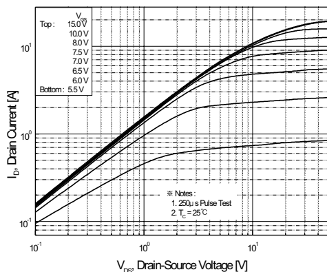
Figure 1. On-Region Characteristic
