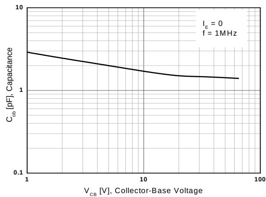
Figure 5. Output Capacitance
