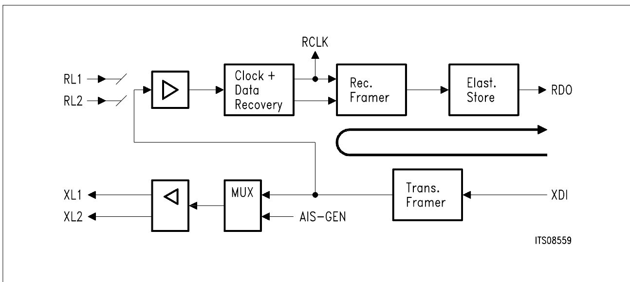
Figure 19 Local Loop
