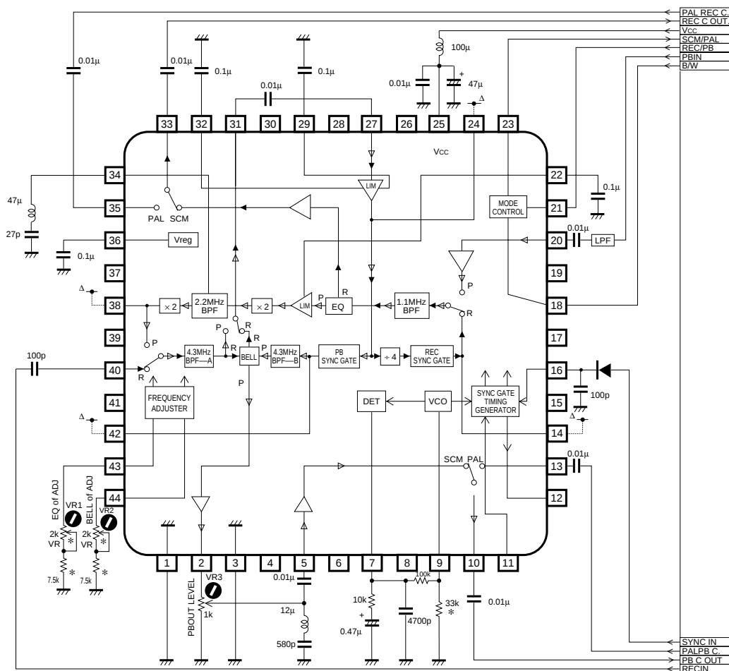
BA7207AK (QFP44)
