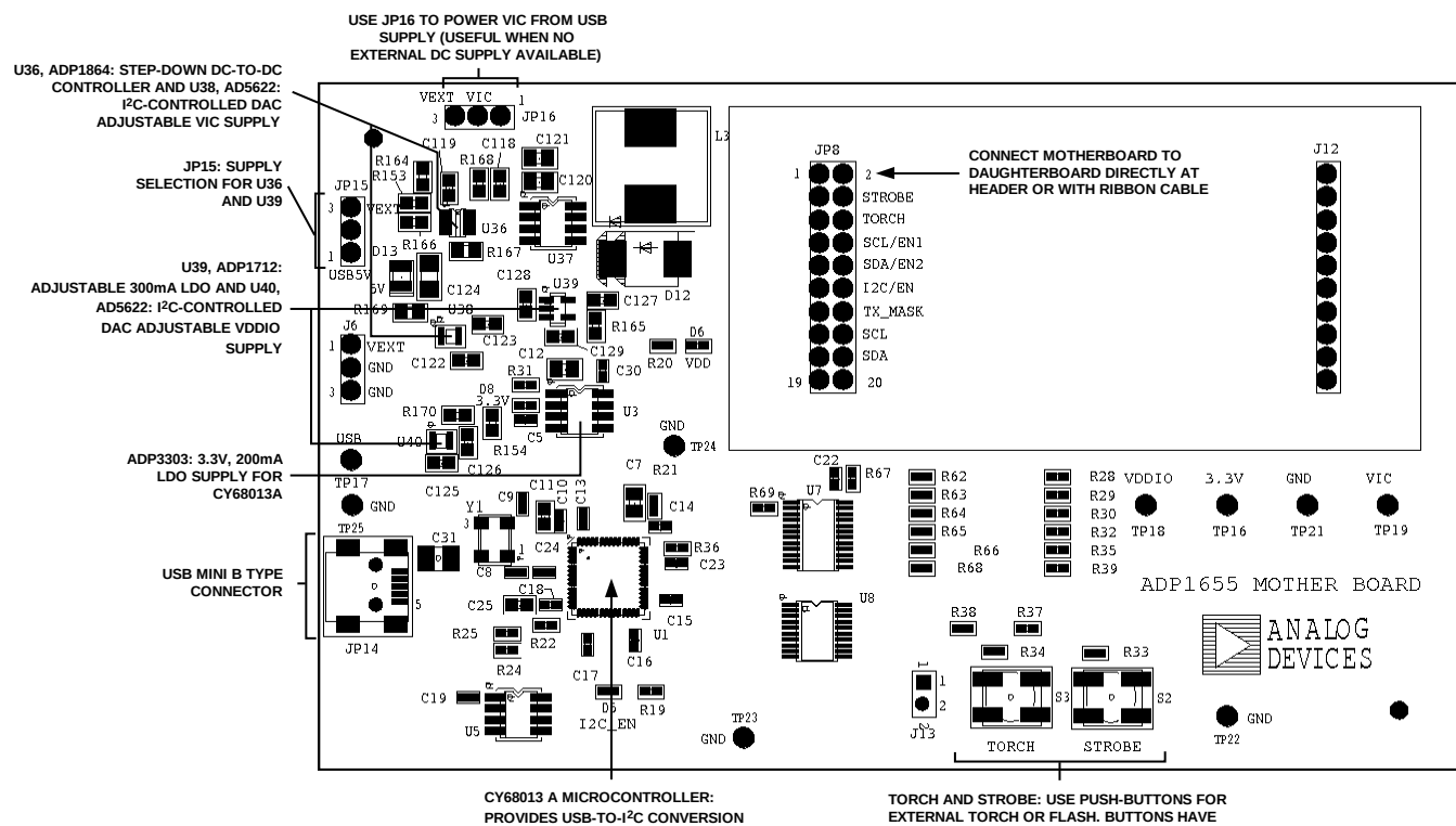
Figure 13. Motherboard
