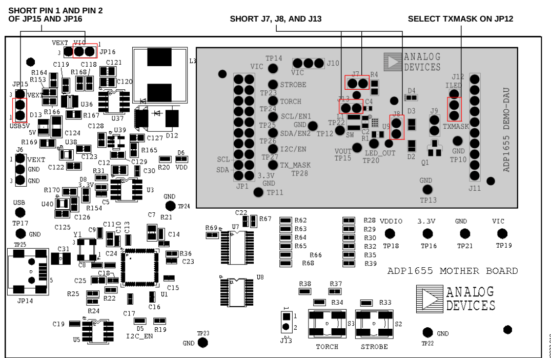
Figure 16. Powering ADP1655 from USB Port
