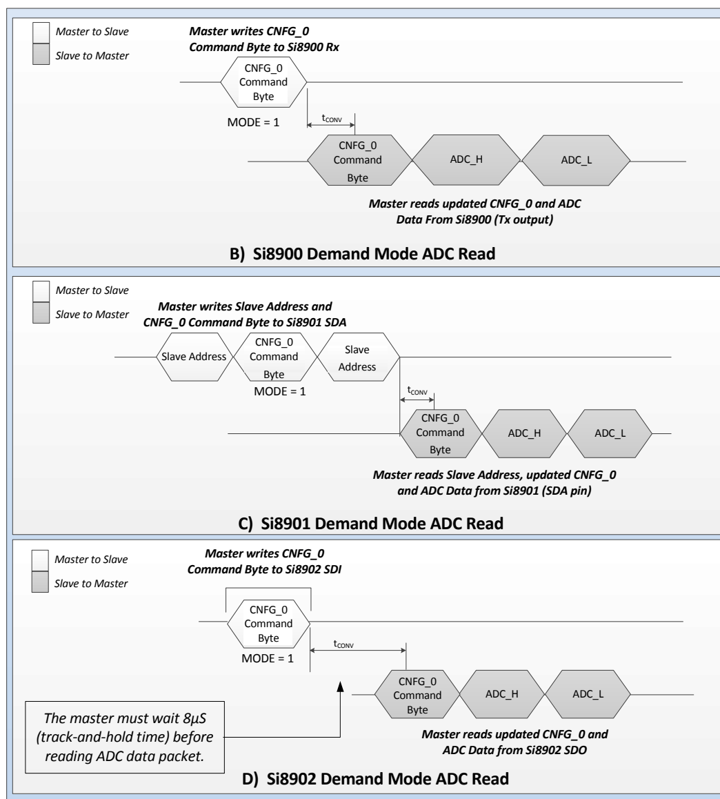
Figure 5. ADC Demand Mode Operation
