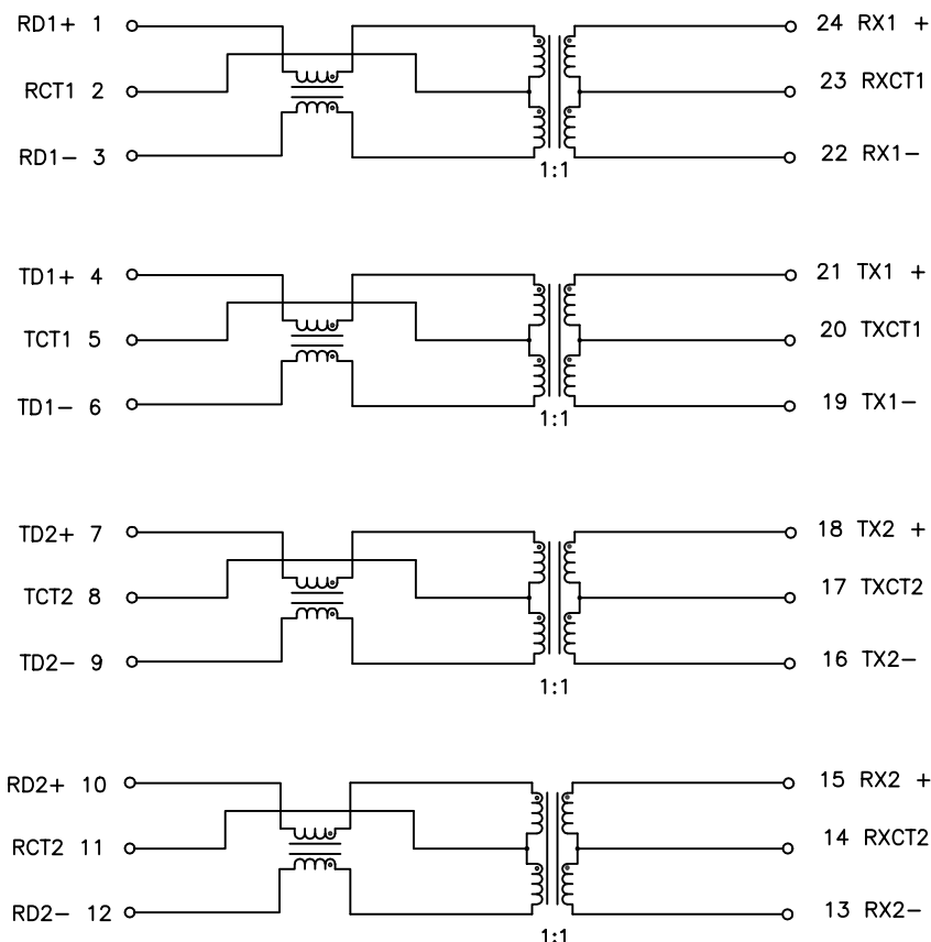
SCHEMATIC
