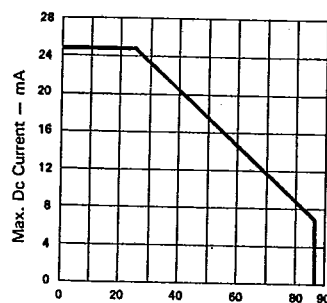
6-133 608 Fig. 4 MAX. ALLOWABLE DC CURRENT PER SEG. Vs AMBIENT TEMPERATURE.
