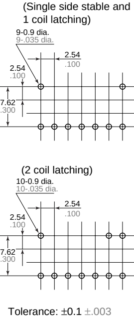
PC board pattern (Copper-side view)
