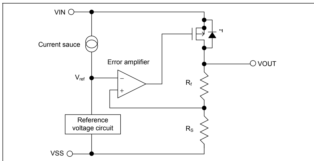
Figure 11 Block diagram
