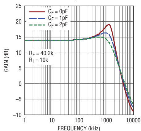
LTC6090-5 Small Signal Frequency Response vs Feedback Capacitance
