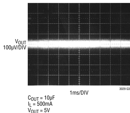
10Hz to 100kHz Output Noise, C_{BYP} = 0.01\mu\text{F}
