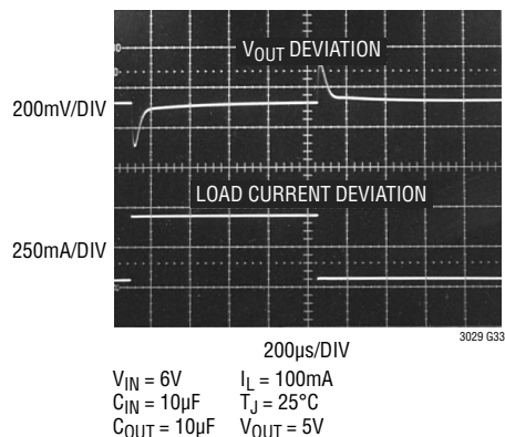
Transient Response, C_{BYP} = 0\text{pF}
