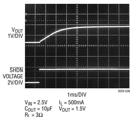
Start-Up Time from Shutdown, C_{BYP} = 0.01\mu\text{F}
