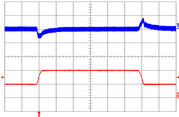
Fig. 2.0V.5: Output voltage response to load current step-change (5A – 10A – 5A) at V_{in} = 48 V. Top trace: output voltage (100 mV/div.). Bottom trace: load current (5 A/div.). Current slew rate: 0.1 A/ \mu s. C_o = 1 \mu F ceramic. Time scale: 0.2 ms/div.
