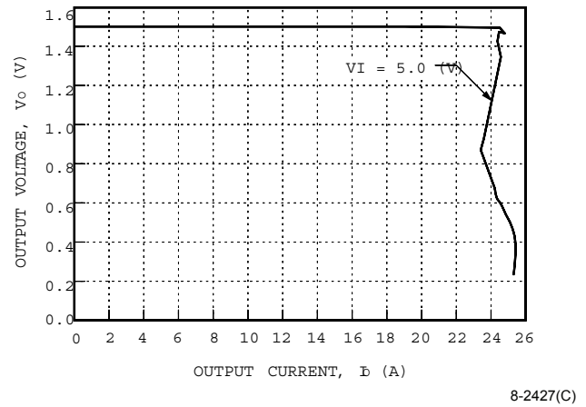
Figure 10. NH050M-L Current Limit, T_A = 25\text{ }^{\circ}\text{C}
