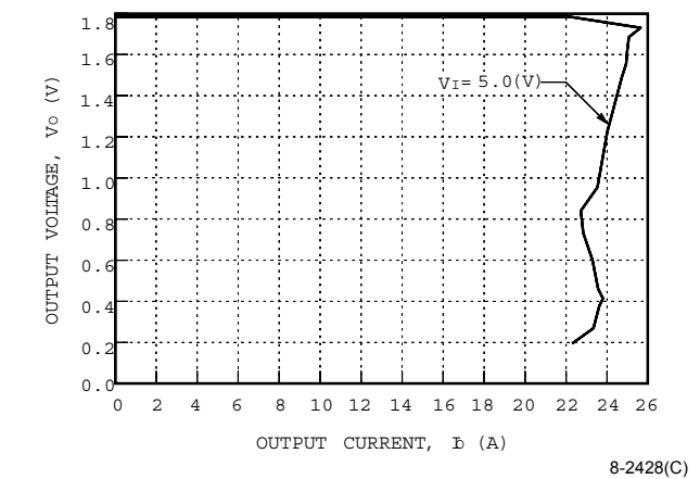
Figure 12. NH050S1R8-L Current Limit, T_A = 25\text{ }^{\circ}\text{C}
