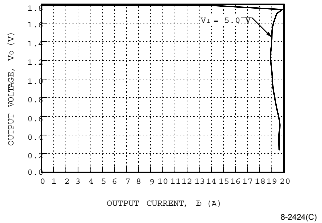
Figure 11. NH033S1R8-L Current Limit, T_A = 25\text{ }^{\circ}\text{C}
