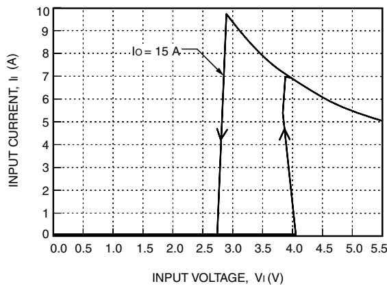
Figure 2. NH050M-L Input Characteristics, T_A = 25\text{ }^{\circ}\text{C}
