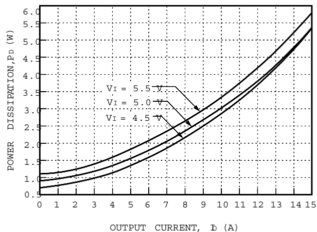
Figure 49. NH050F-L Typical Power Dissipation vs. Output Current, T_A = 25\text{ °C}
