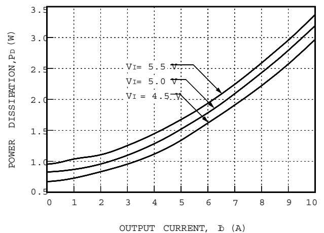
Figure 46. NH033G-L Typical Power Dissipation vs. Output Current, T_A = 25\text{ °C}
