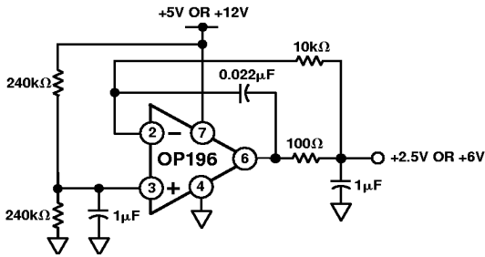
Figure 41. A Micropower False-Ground Generator
