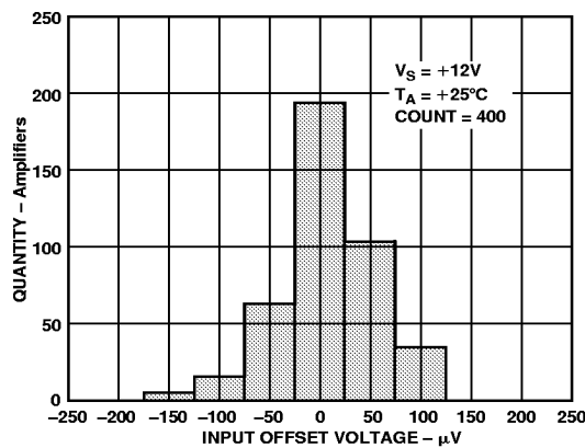
Figure 3. Input Offset Voltage Distribution
