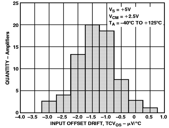
Figure 4. Input Offset Voltage Distribution (TCVOS)
