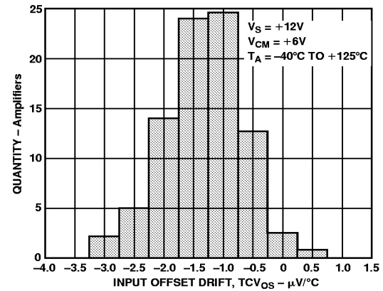
Figure 5. Input Offset Voltage Distribution (TCVOS)
