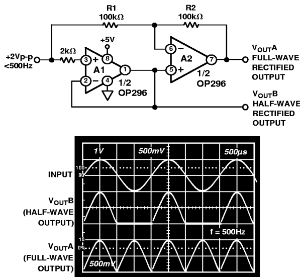
Figure 42. Single-Supply Half-Wave and Full-Wave Rectifiers Using an OP296
