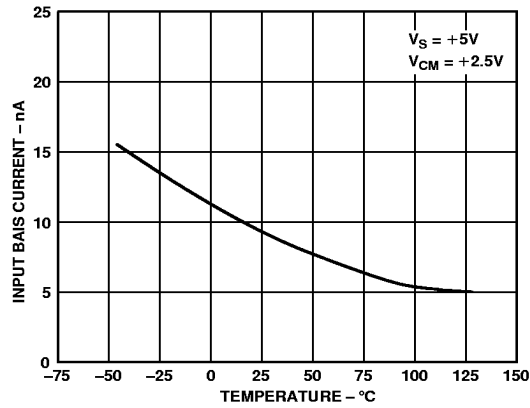
Figure 7. Input Bias Current vs. Temperature
