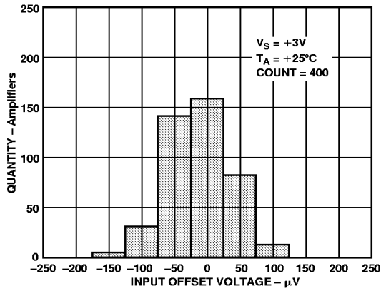
Figure 1. Input Offset Voltage Distribution
