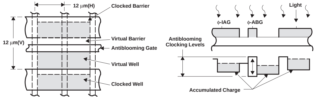
Figure 1. Charge-Accumulation Process
