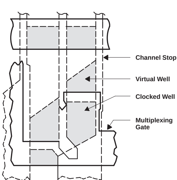
Figure 3. Multiplexing-Gate Layout
