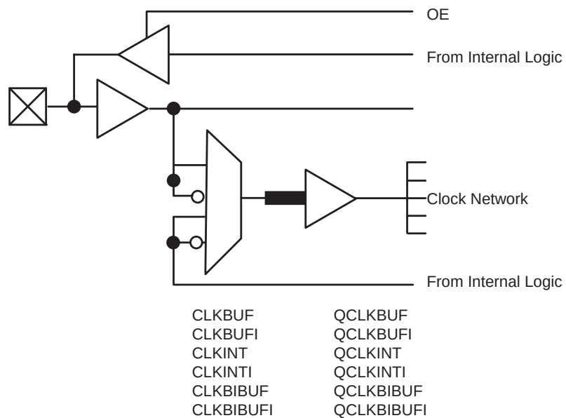
Figure 2-21 • Routed and Quadrant Clock Buffers in RTSX72SU
