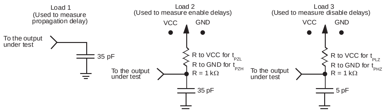
Figure 2-6 • AC Test Loads
