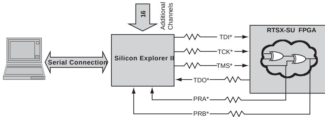
Figure 1-5 • Probe Setup
