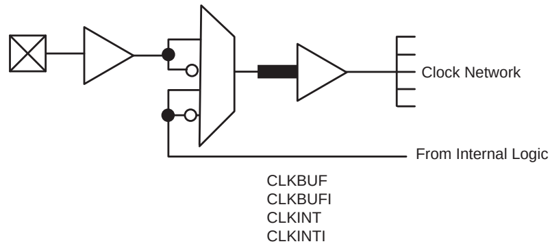
Figure 2-20 • Routed Clock Buffers in RTSX32SU
