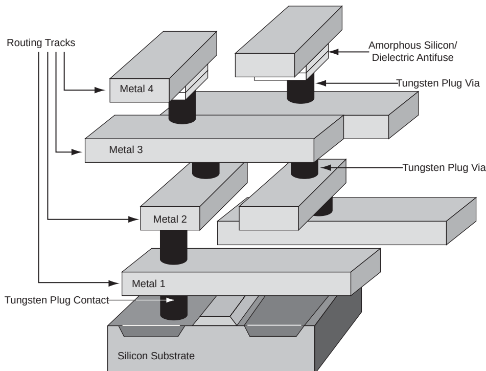
Figure 1-1 • RTSX-SU Family Interconnect Elements
