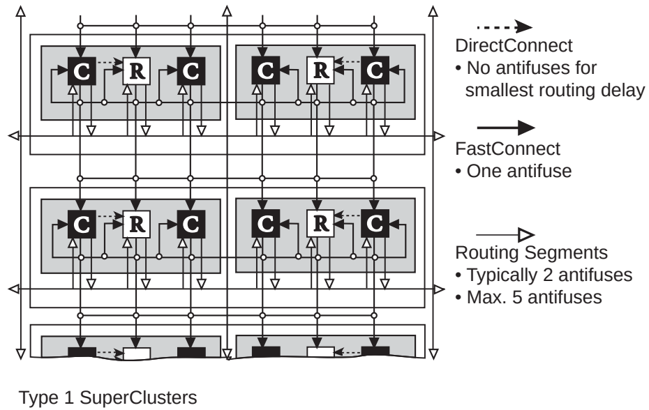
Figure 1-3 • DirectConnect and FastConnect for SuperCluster 1's
