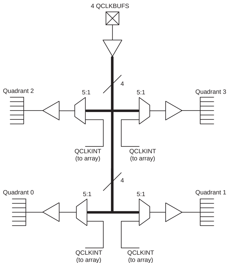
Figure 2-18 • RTSX-SU QCLK Structure
