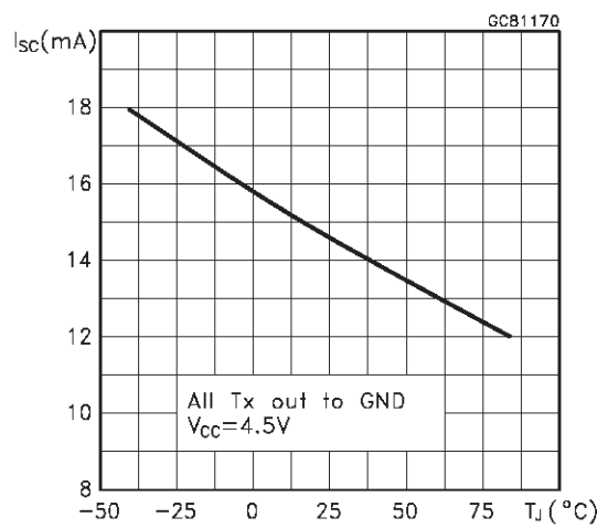
High Level Trasmitter Output Short Circuit Current vs Temperature
