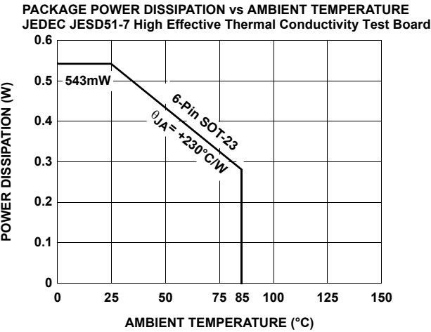
FIGURE 25. PACKAGE POWER DISSIPATION vs AMBIENT TEMPERATURE
