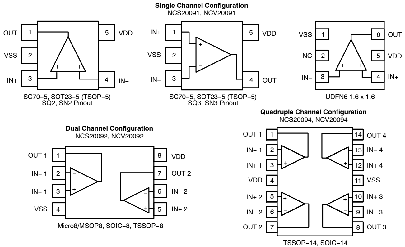
Figure 1. Pin Connections
