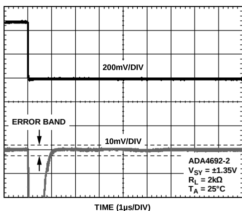
Figure 52. Negative Settling Time to 0.1%
