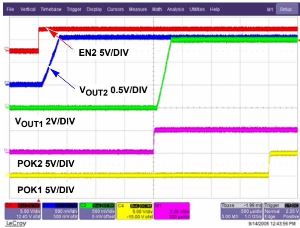
FIGURE 59. DELAYED START-UP ( V_{OUT1} = 1.5V , V_{OUT2} = 1.05V , EN1 = REF )
