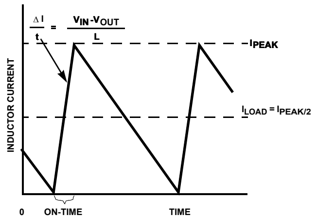
FIGURE 71. ULTRASONIC CURRENT WAVEFORMS
