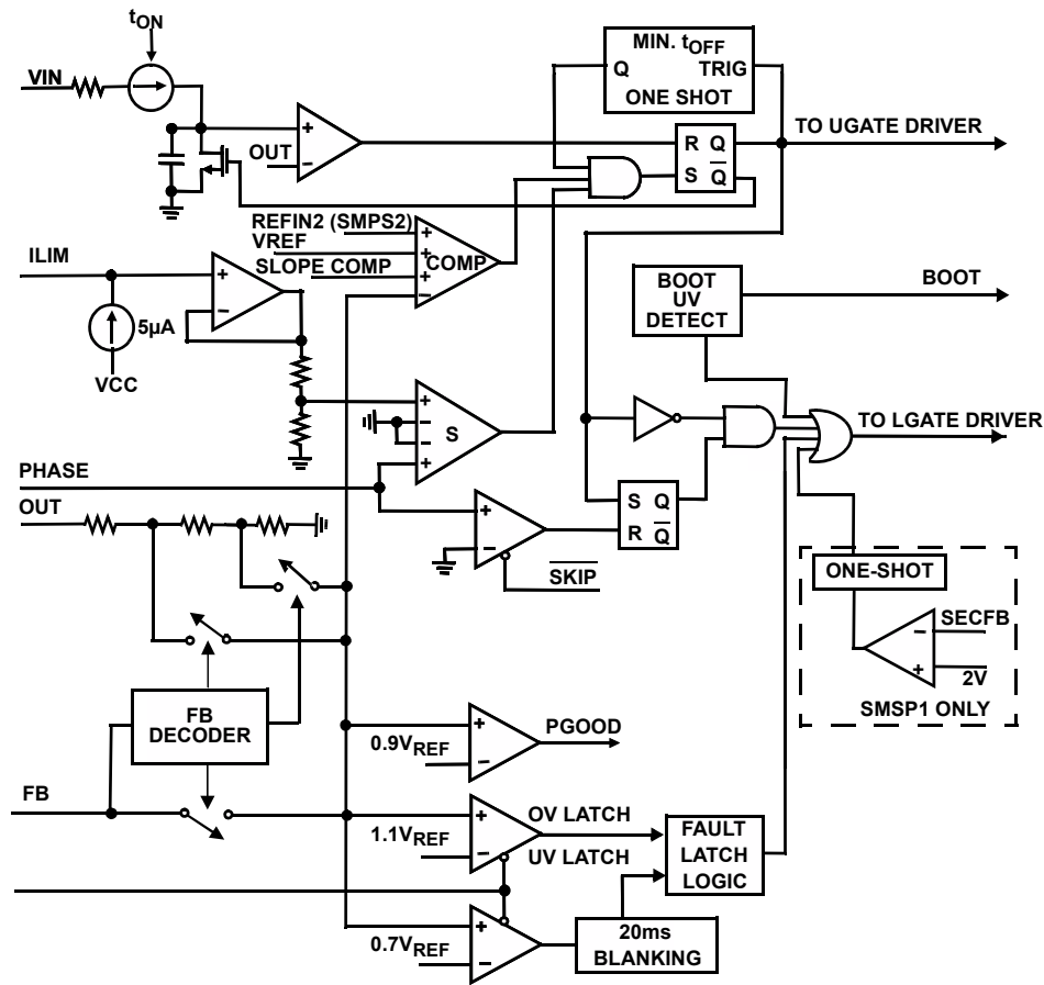
FIGURE 70. PWM CONTROLLER (ONE SIDE ONLY)
