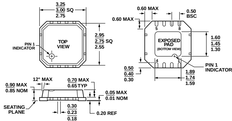
Figure 54. 8-Lead Lead Frame Chip Scale Package [LFCSP_VD] 3 mm x 3 mm Body, Very Thin, Dual Lead (CP-8-2) Dimensions shown in millimeters
