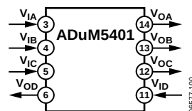
Figure 2. ADuM5401
