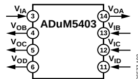
Figure 4. ADuM5403
