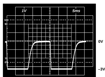
Figure 10. Enable/Disable Time Under Full Load
