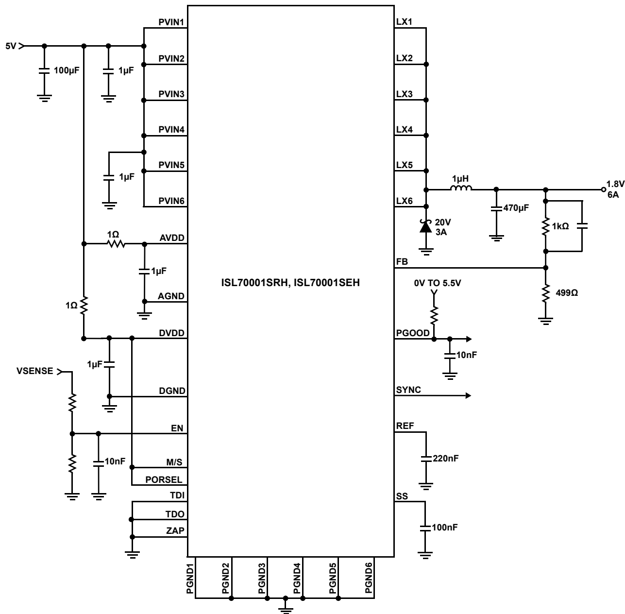
FIGURE 4. 5V INPUT SUPPLY VOLTAGE WITH MASTER MODE SYNCHRONIZATION
