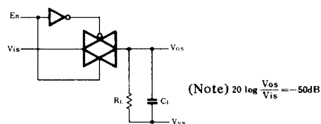
Fig. 2 Sine Wave Distortion, Feedthrough Test Circuit
