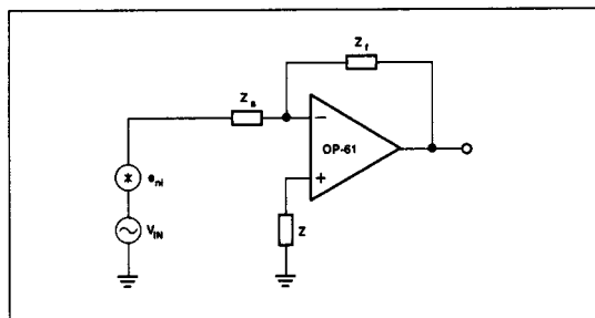
FIGURE 17: Equivalent Noise Model, Where All Noise Contributions are Lumped Into e_{ni}
