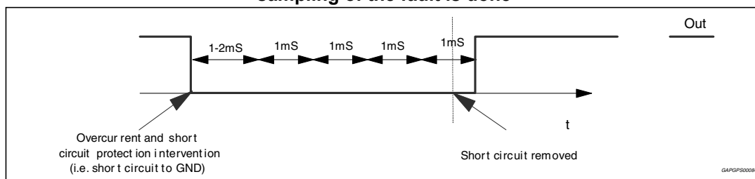
Figure 30. Restart timing with diagnostic enable (permanent)
