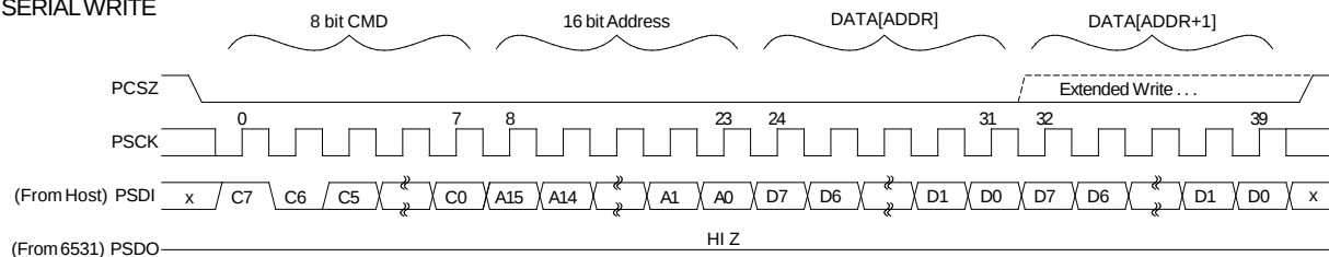
Figure 4: SPI Slave Port: Typical Read and Write Operations
