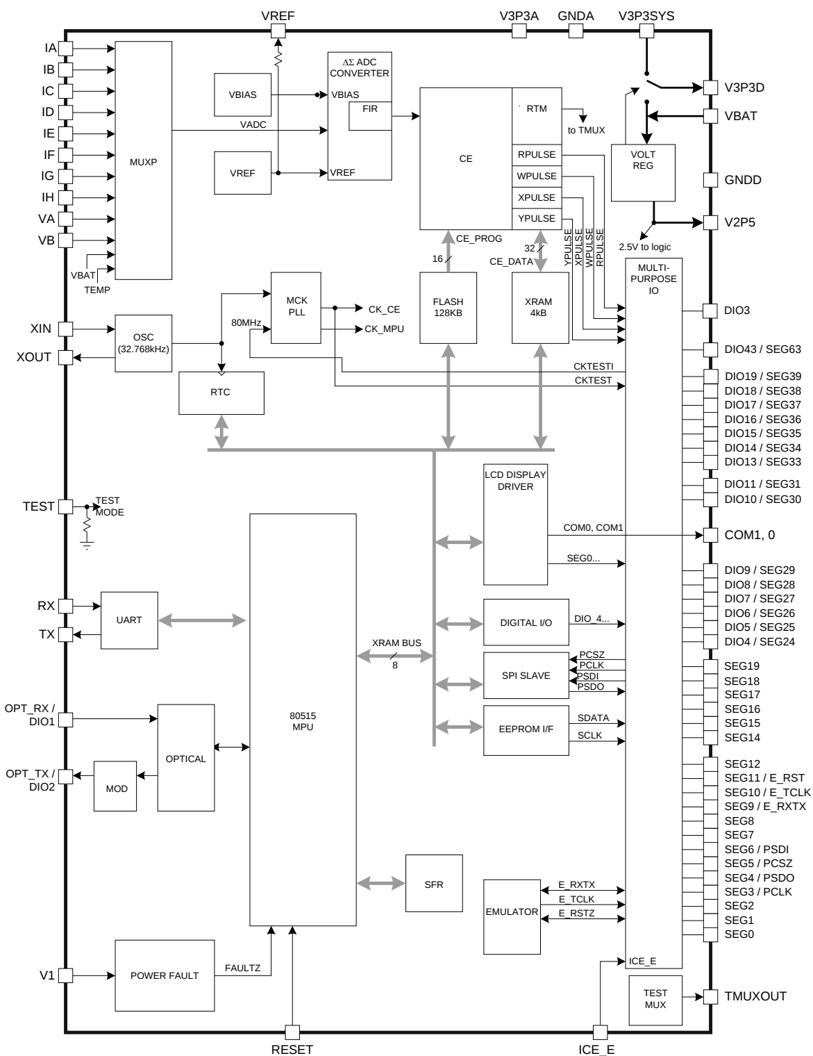
Figure 1: 78M6618 IC Functional Block Diagram
