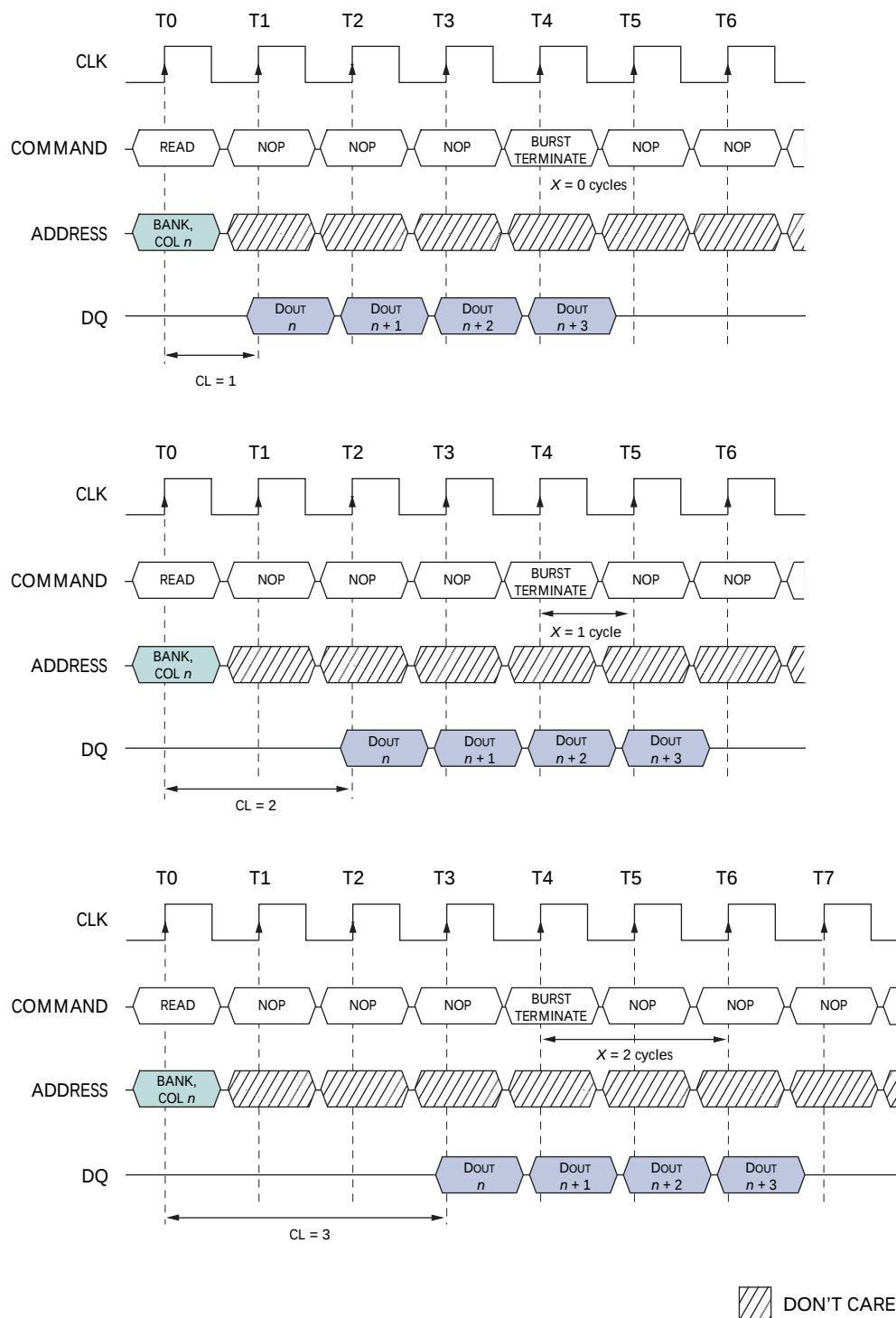
Figure 15: Terminating a READ Burst
