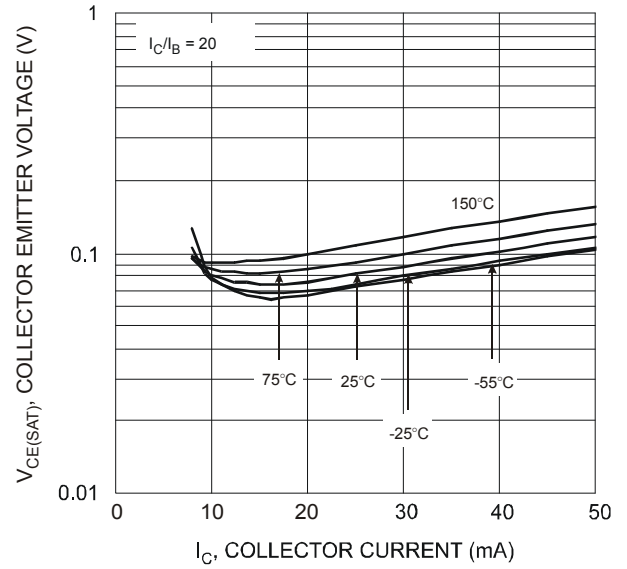
Fig. 4 V_{CE(SAT)} vs. I_C
