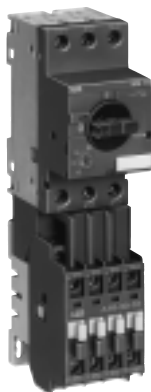
MS 116 with A-contactor
