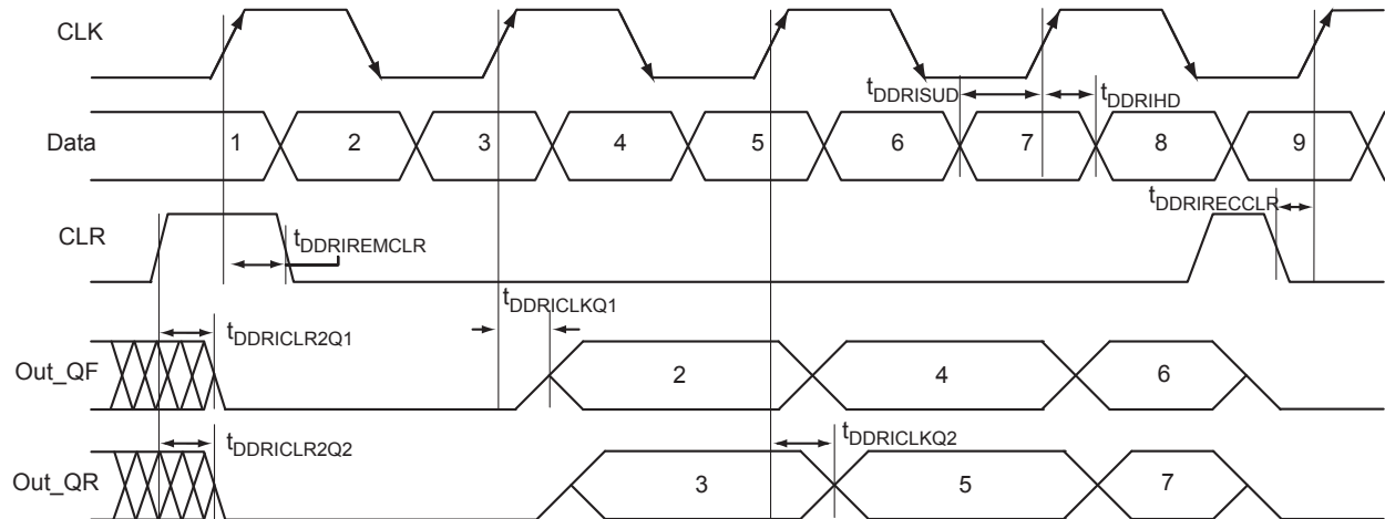
Figure 2-22 • Input DDR Timing Diagram
